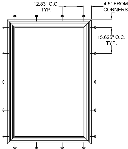
TYPICAL ELEVATION WITH FASTENER SPACING
